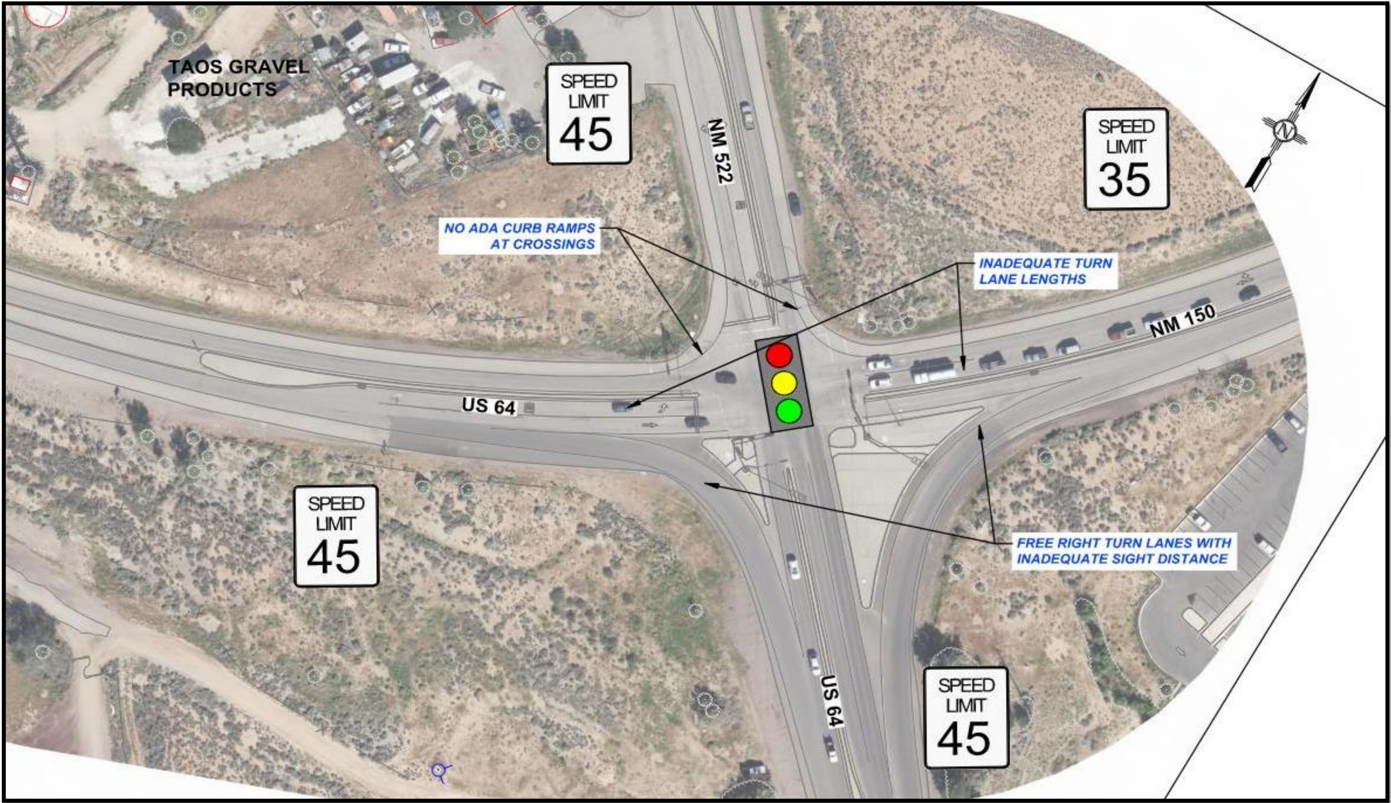
Alternative 1: No Build
