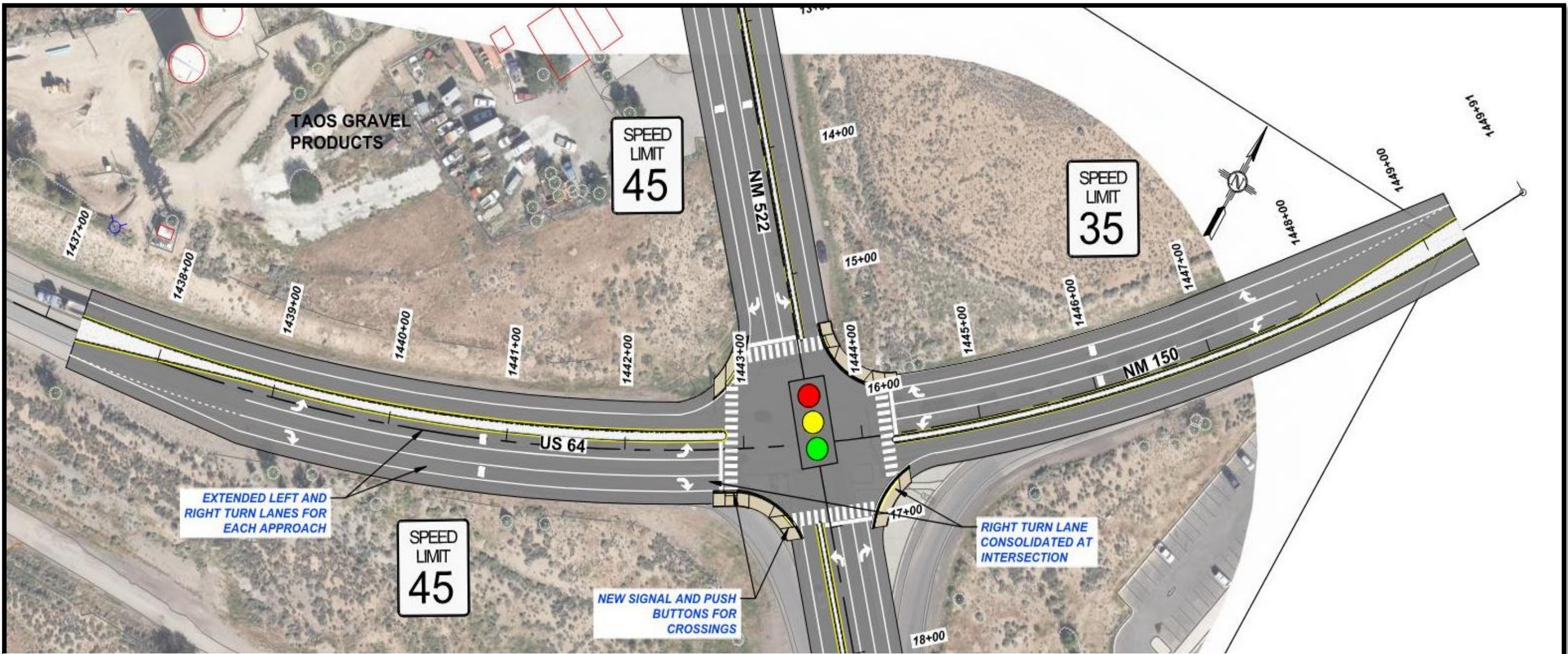
Alternative 2: Signalized Intersection Reconstruction
