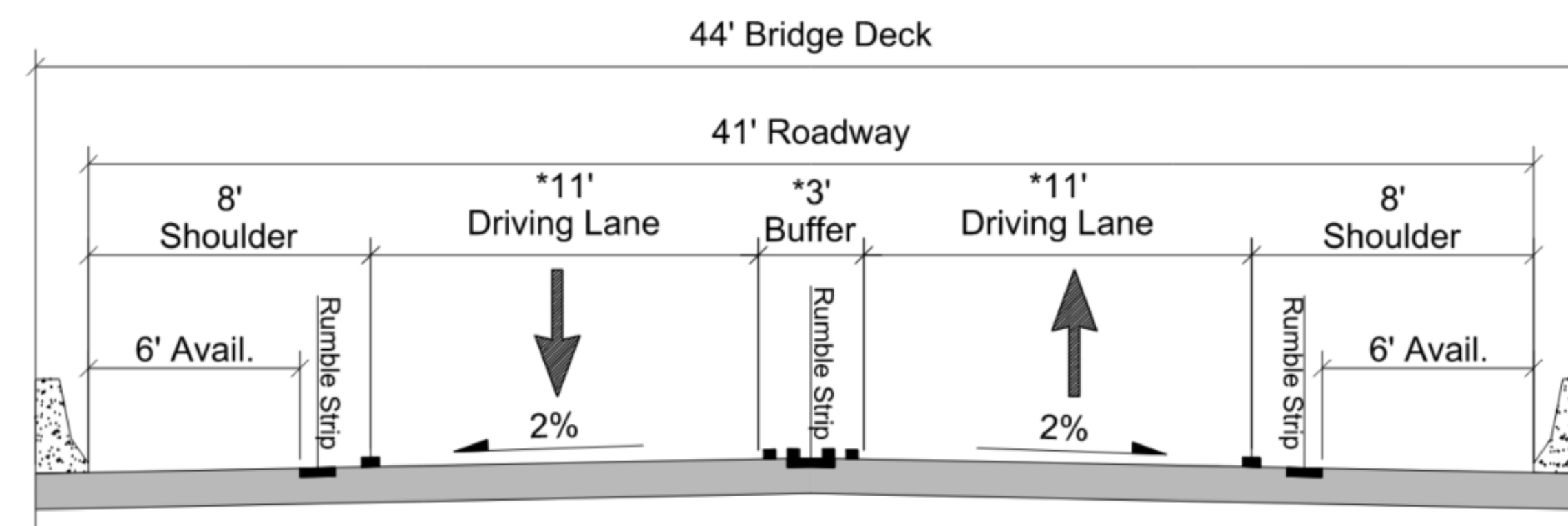
Alternative 2: Full Reconstruction
